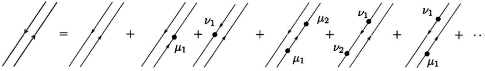
FIG. 1. Wine expansion. The thick lines are expanded into thin lines, with the blobs representing \mathcal{A} fields.
